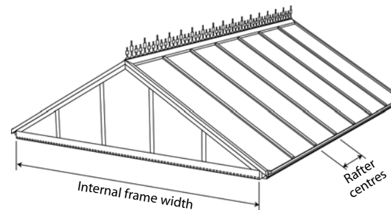
Maximum Duo pitch internal frame width (mm)
