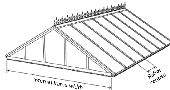
Maximum Duo pitch internal frame width (mm)
